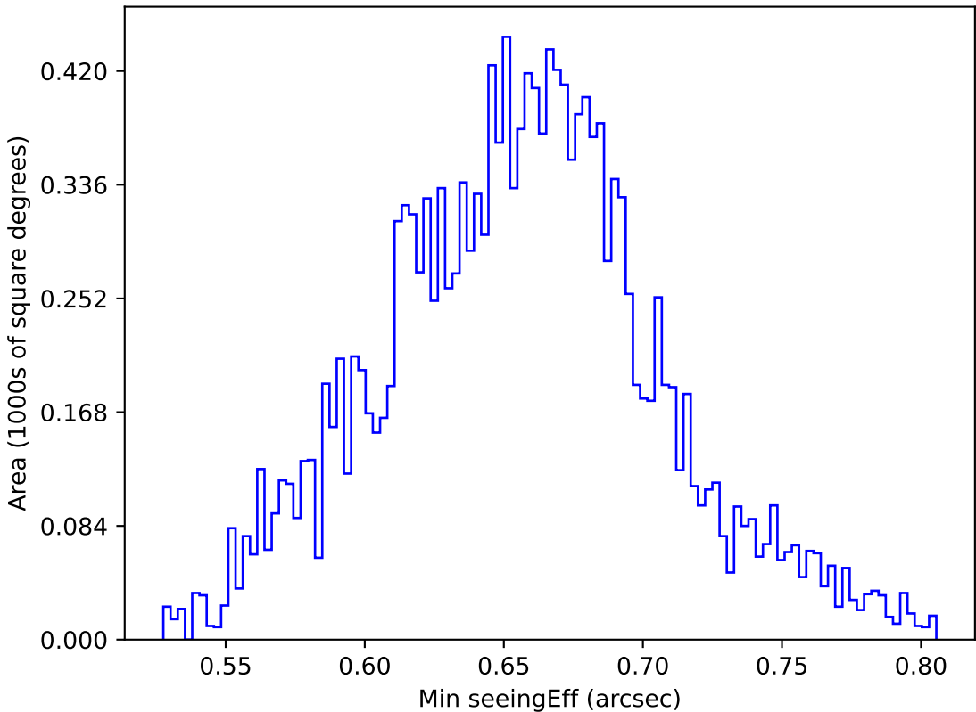
too_elab_r256_d3_griz_v3.4_10yrs WFD g band: Min seeingEff
