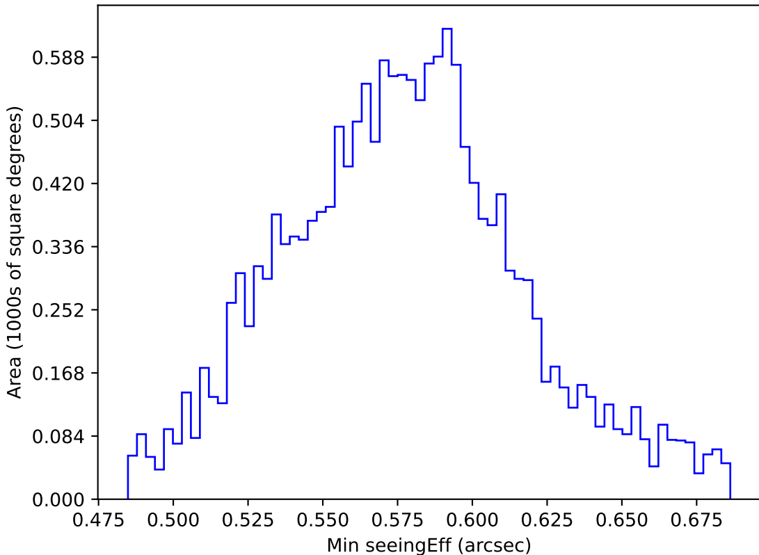
too_elab_r256_d3_griz_v3.4_10yrs WFD all bands: Min seeingEff
