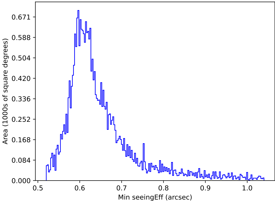
too_elab_r256_d3_griz_v3.4_10yrs All sky z band: Min seeingEff
