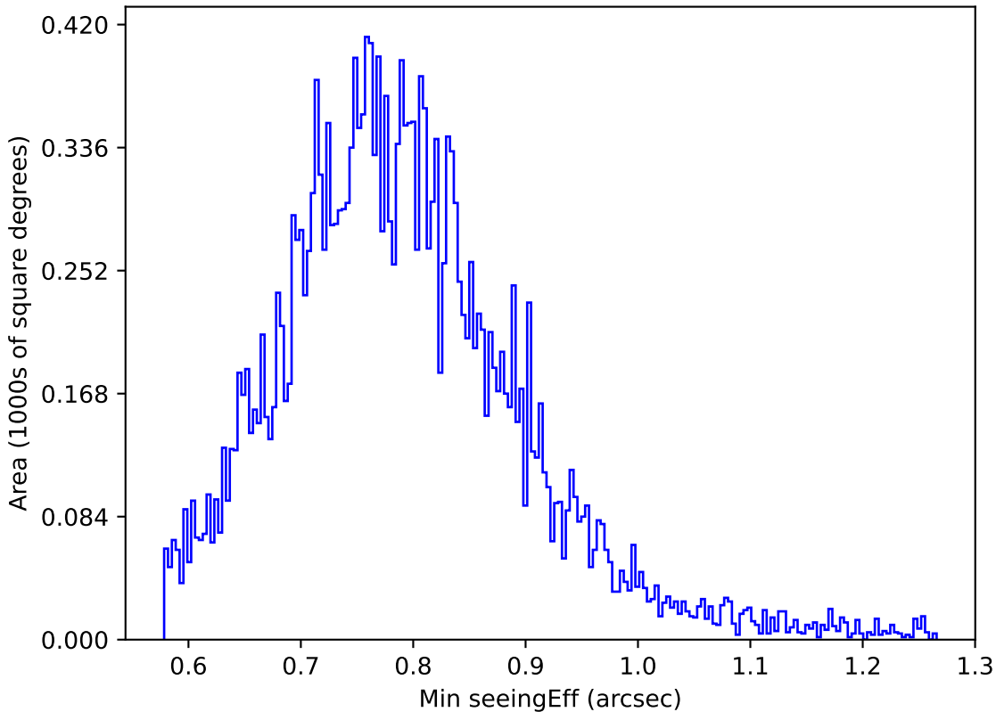
too_elab_r256_d3_griz_v3.4_10yrs All sky u band: Min seeingEff
