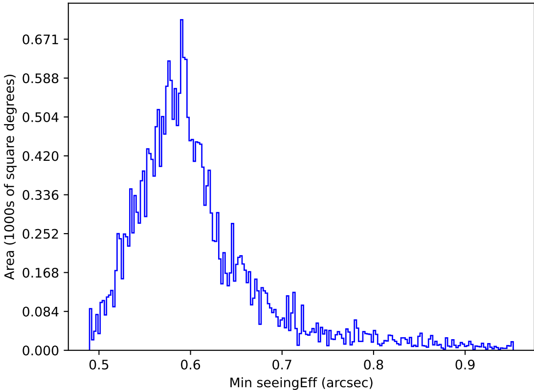
too_elab_r256_d3_griz_v3.4_10yrs All sky all bands: Min seeingEff
