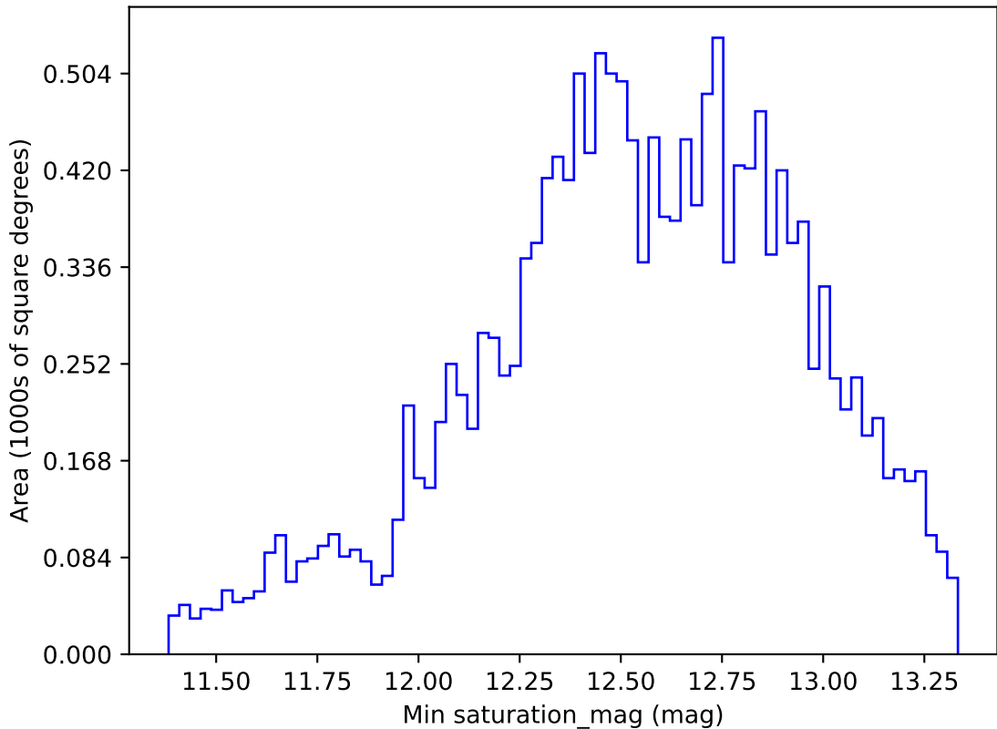
too_elab_r256_d3_griz_v3.4_10yrs WFD r band: Min saturation_mag
