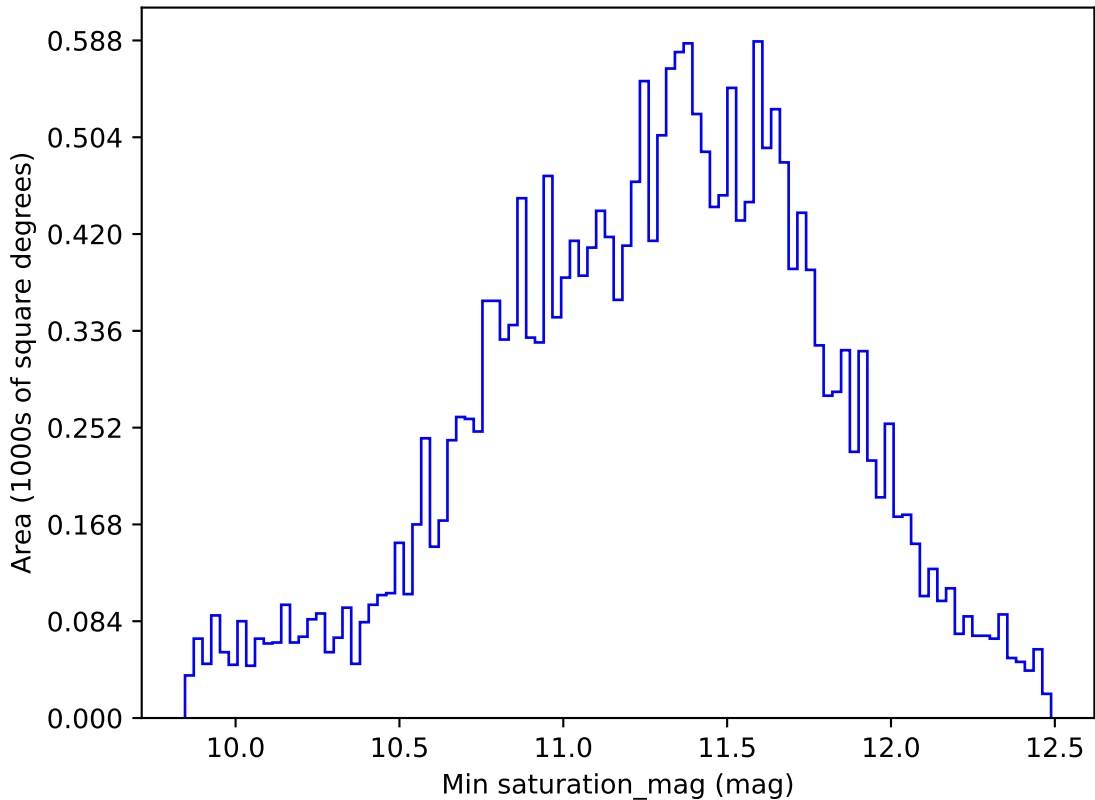
too_elab_r256_d3_griz_v3.4_10yrs All sky y band: Min saturation_mag
