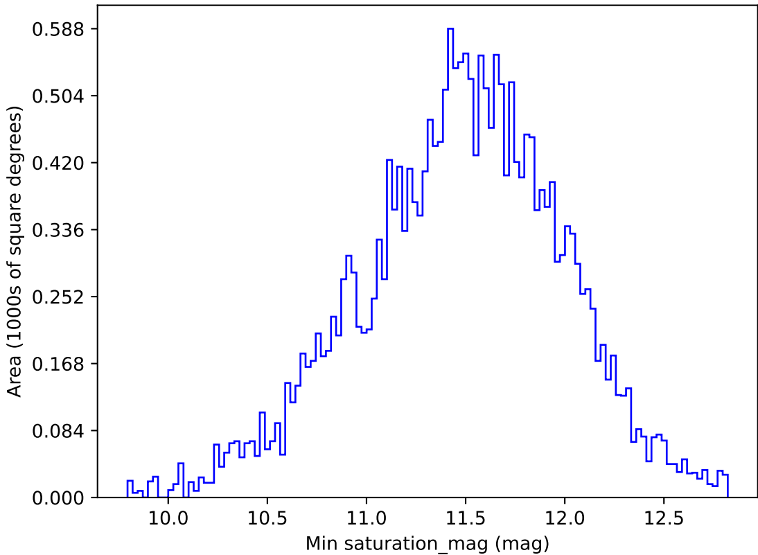
too_elab_r256_d3_griz_v3.4_10yrs All sky u band: Min saturation_mag
