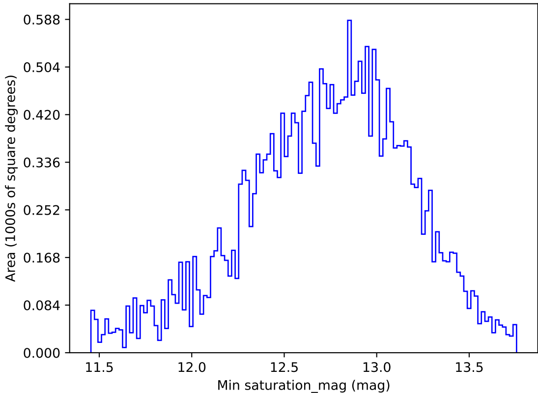
too_elab_r256_d3_griz_v3.4_10yrs All sky g band: Min saturation_mag
