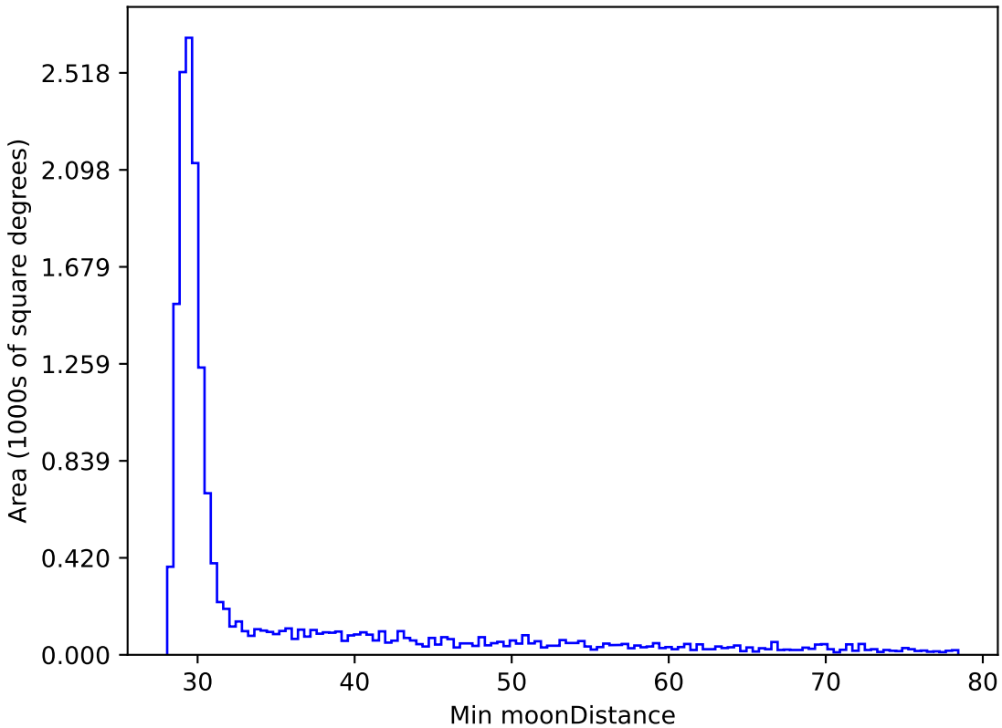
too_elab_r256_d3_griz_v3.4_10yrs WFD y band: Min moonDistance
