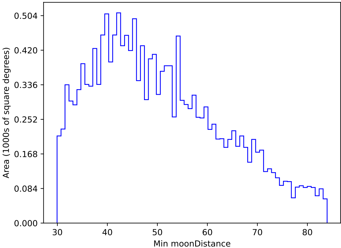
too_elab_r256_d3_griz_v3.4_10yrs WFD u band: Min moonDistance
