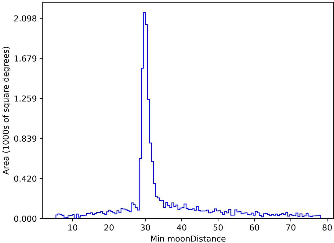
too_elab_r256_d3_griz_v3.4_10yrs WFD i band: Min moonDistance
