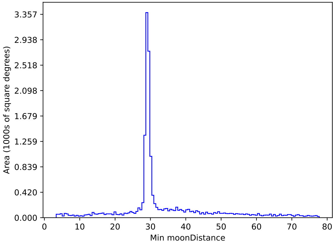
too_elab_r256_d3_griz_v3.4_10yrs WFD all bands: Min moonDistance
