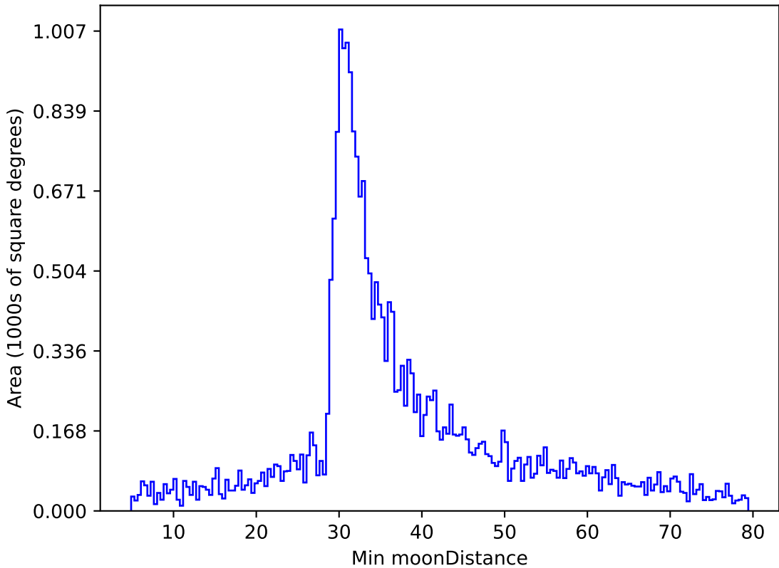
too_elab_r256_d3_griz_v3.4_10yrs All sky r band: Min moonDistance
