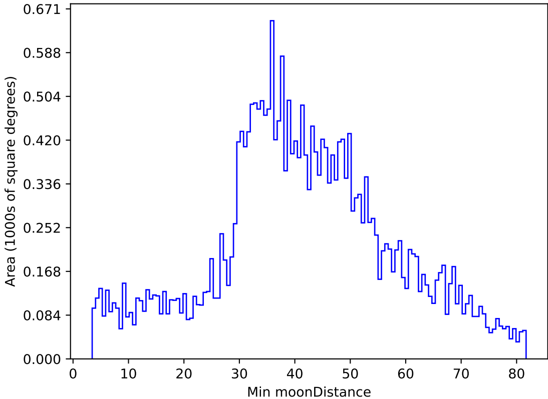
too_elab_r256_d3_griz_v3.4_10yrs All sky g band: Min moonDistance
