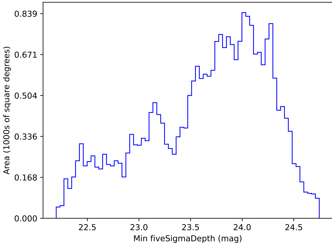
too_elab_r256_d3_griz_v3.4_10yrs Yr 1 g band: Min fiveSigmaDepth
