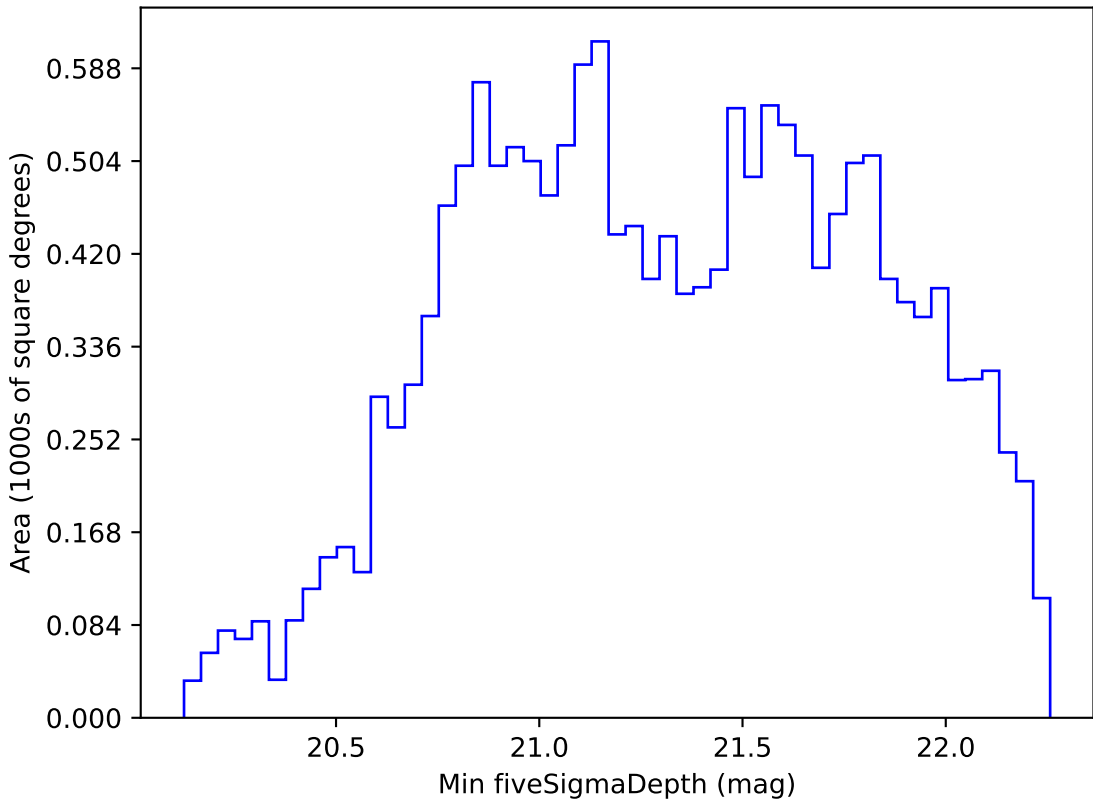
too_elab_r256_d3_griz_v3.4_10yrs WFD z band: Min fiveSigmaDepth
