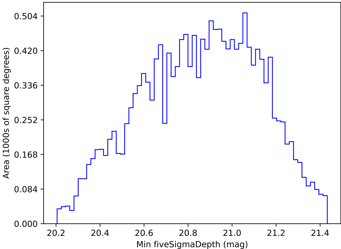
too_elab_r256_d3_griz_v3.4_10yrs WFD y band: Min fiveSigmaDepth
