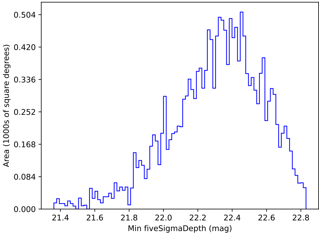
too_elab_r256_d3_griz_v3.4_10yrs WFD u band: Min fiveSigmaDepth
