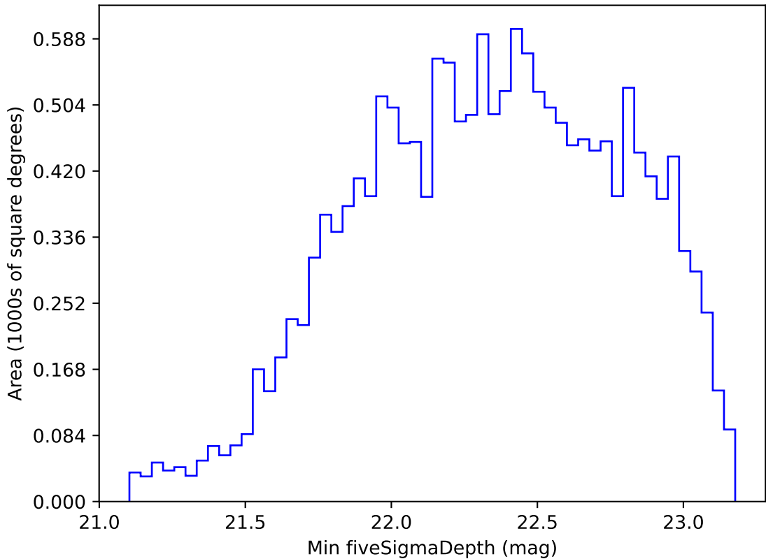
too_elab_r256_d3_griz_v3.4_10yrs WFD r band: Min fiveSigmaDepth
