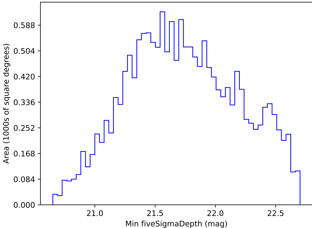
too_elab_r256_d3_griz_v3.4_10yrs WFD i band: Min fiveSigmaDepth
