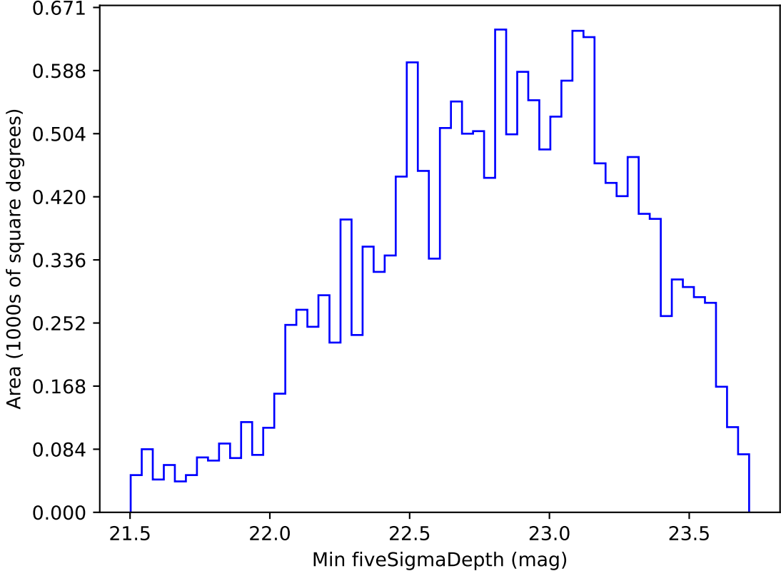
too_elab_r256_d3_griz_v3.4_10yrs WFD g band: Min fiveSigmaDepth
