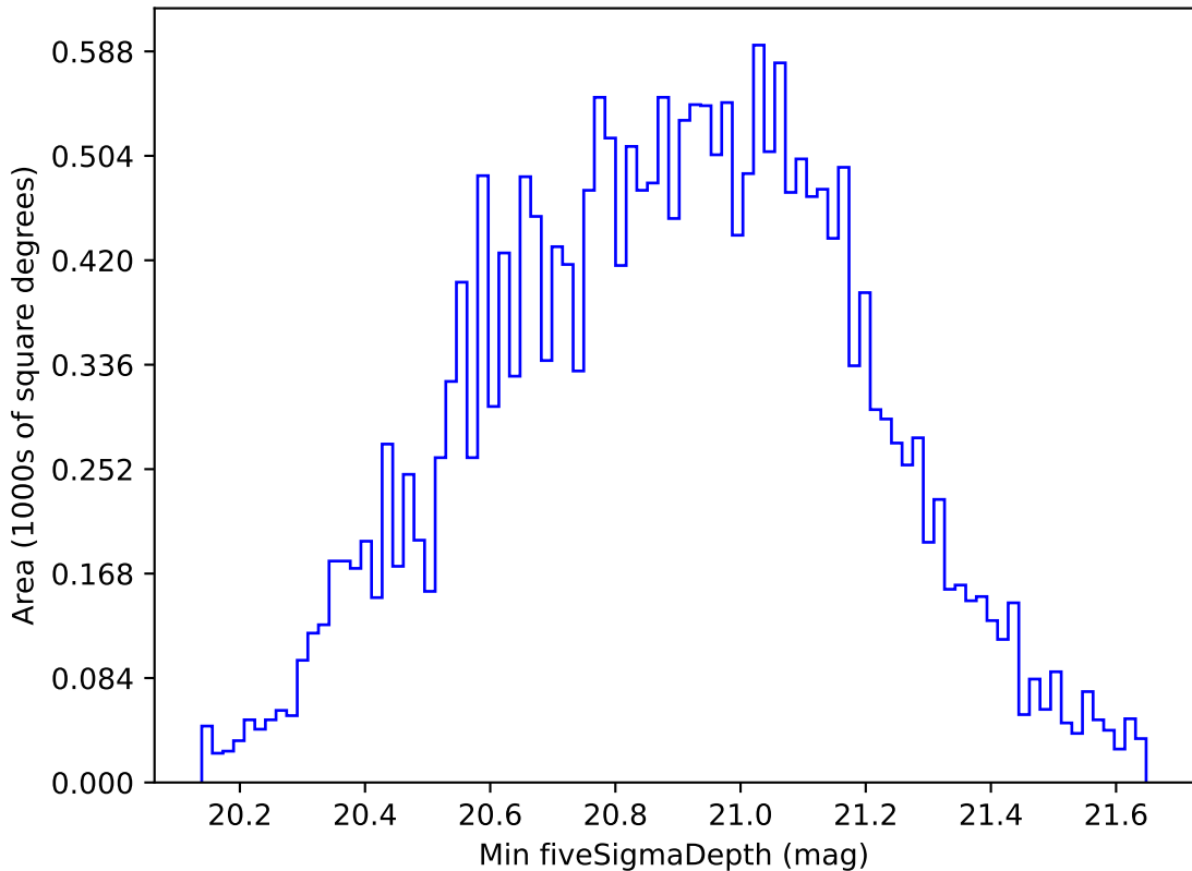
too_elab_r256_d3_griz_v3.4_10yrs All sky y band: Min fiveSigmaDepth
