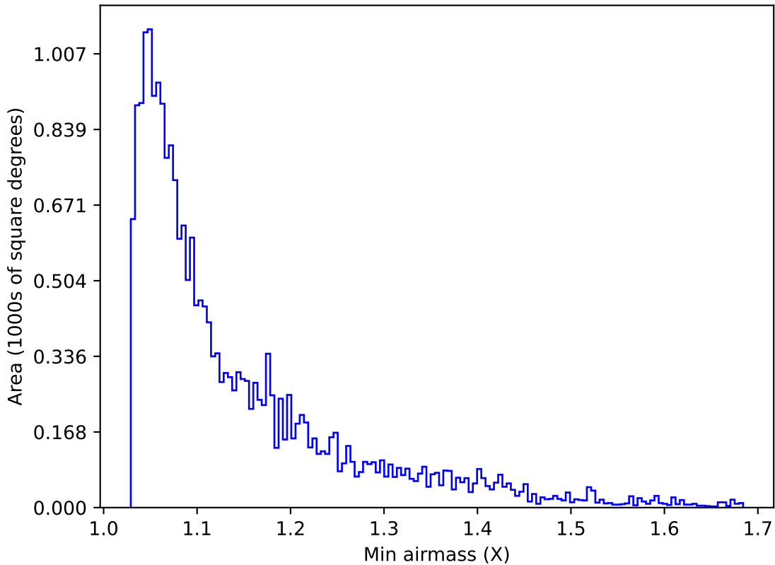
too_elab_r256_d3_griz_v3.4_10yrs Yr 1 u band: Min airmass
