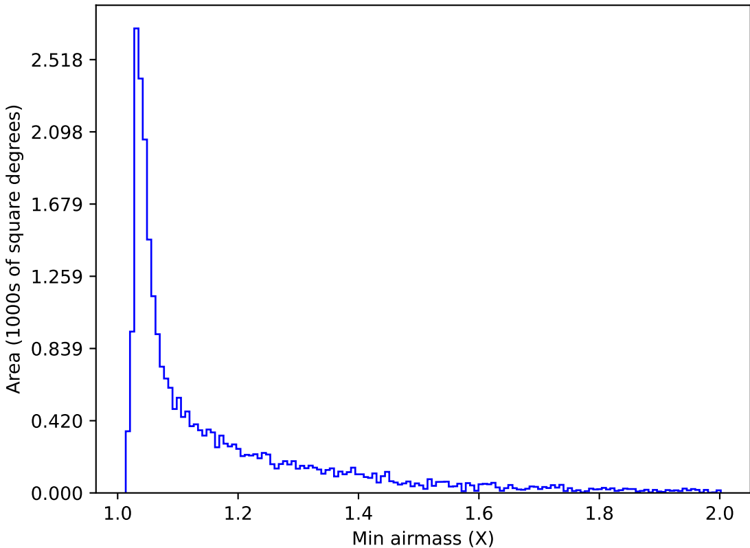
too_elab_r256_d3_griz_v3.4_10yrs Yr 1 r band: Min airmass
