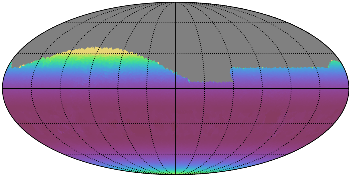
too_elab_r256_d3_griz_v3.4_10yrs Yr 1 all bands: Min airmass
