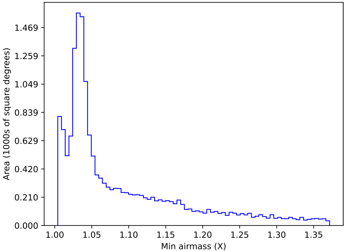
too_elab_r256_d3_griz_v3.4_10yrs WFD g band: Min airmass
