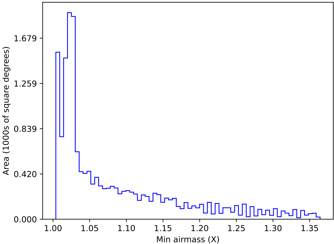
too_elab_r256_d3_griz_v3.4_10yrs WFD all bands: Min airmass
