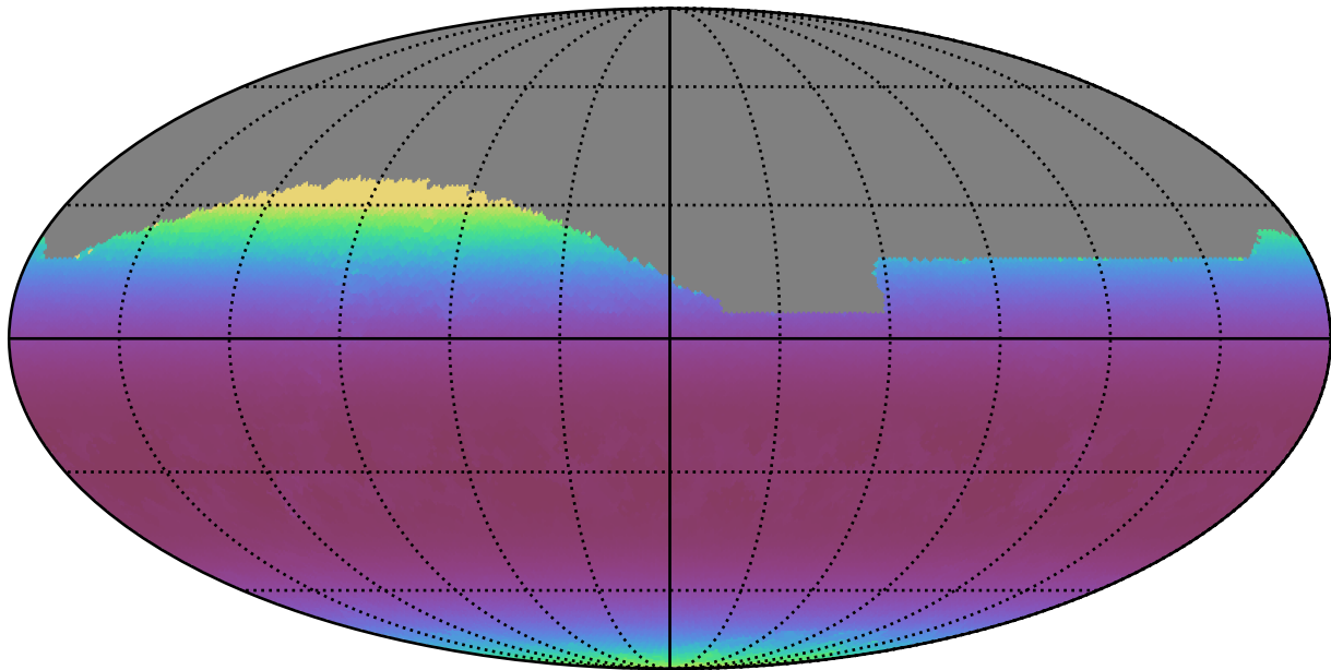
too_elab_r256_d3_griz_v3.4_10yrs All sky z band: Min airmass
