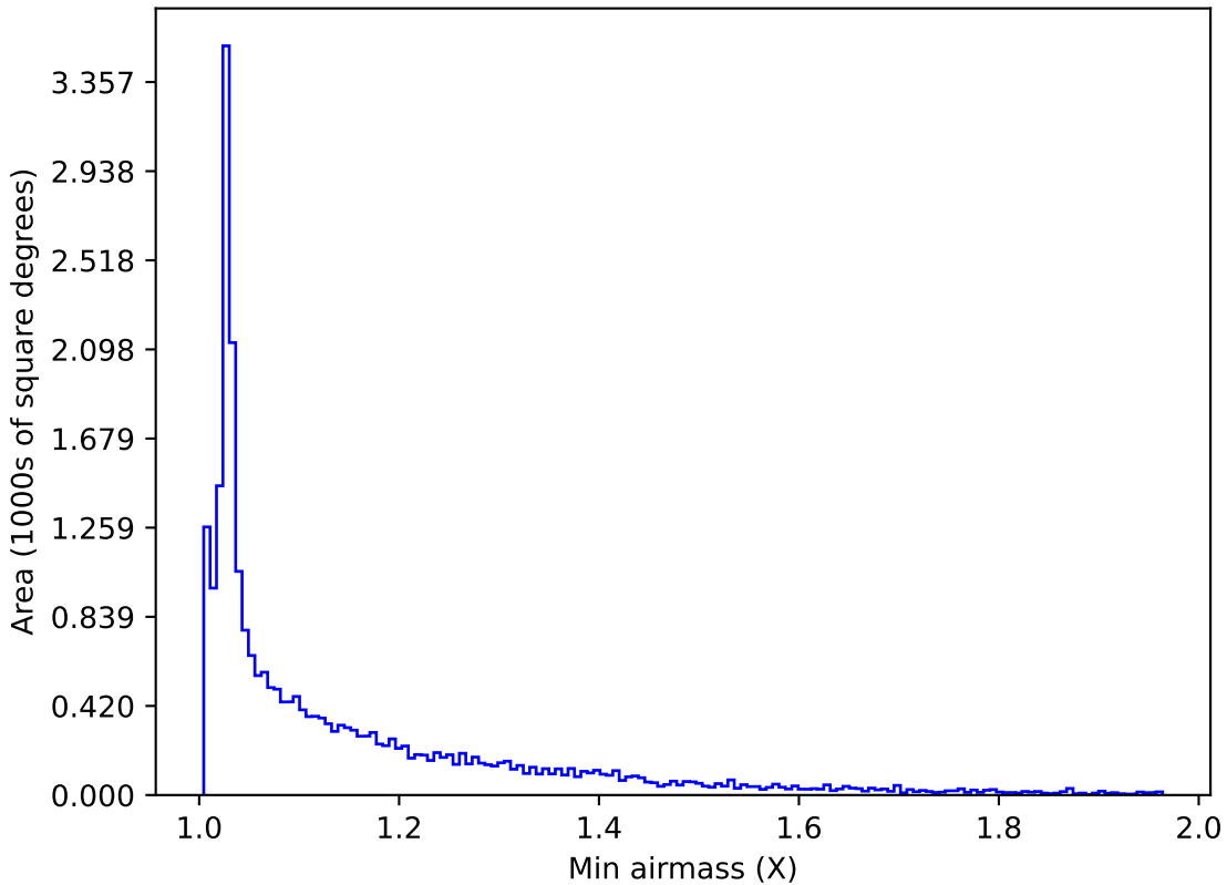
too_elab_r256_d3_griz_v3.4_10yrs All sky z band: Min airmass
