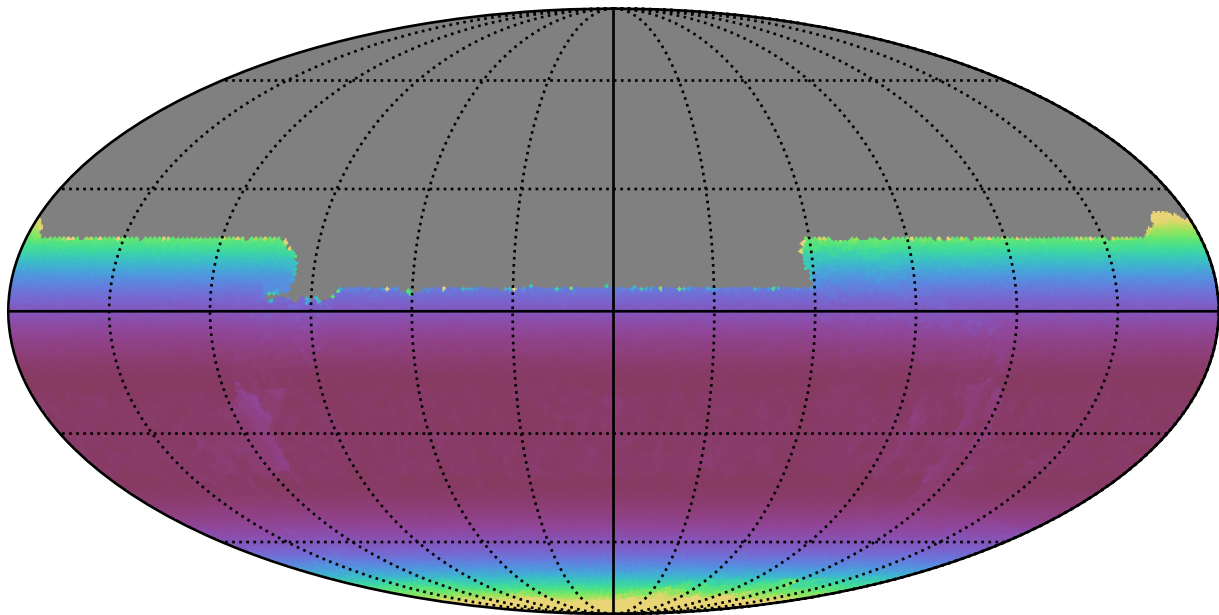
too_elab_r256_d3_griz_v3.4_10yrs All sky y band: Min airmass
