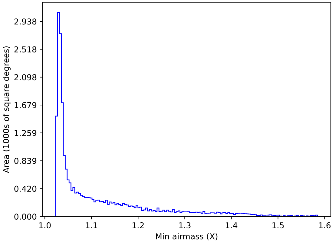
too_elab_r256_d3_griz_v3.4_10yrs All sky y band: Min airmass
