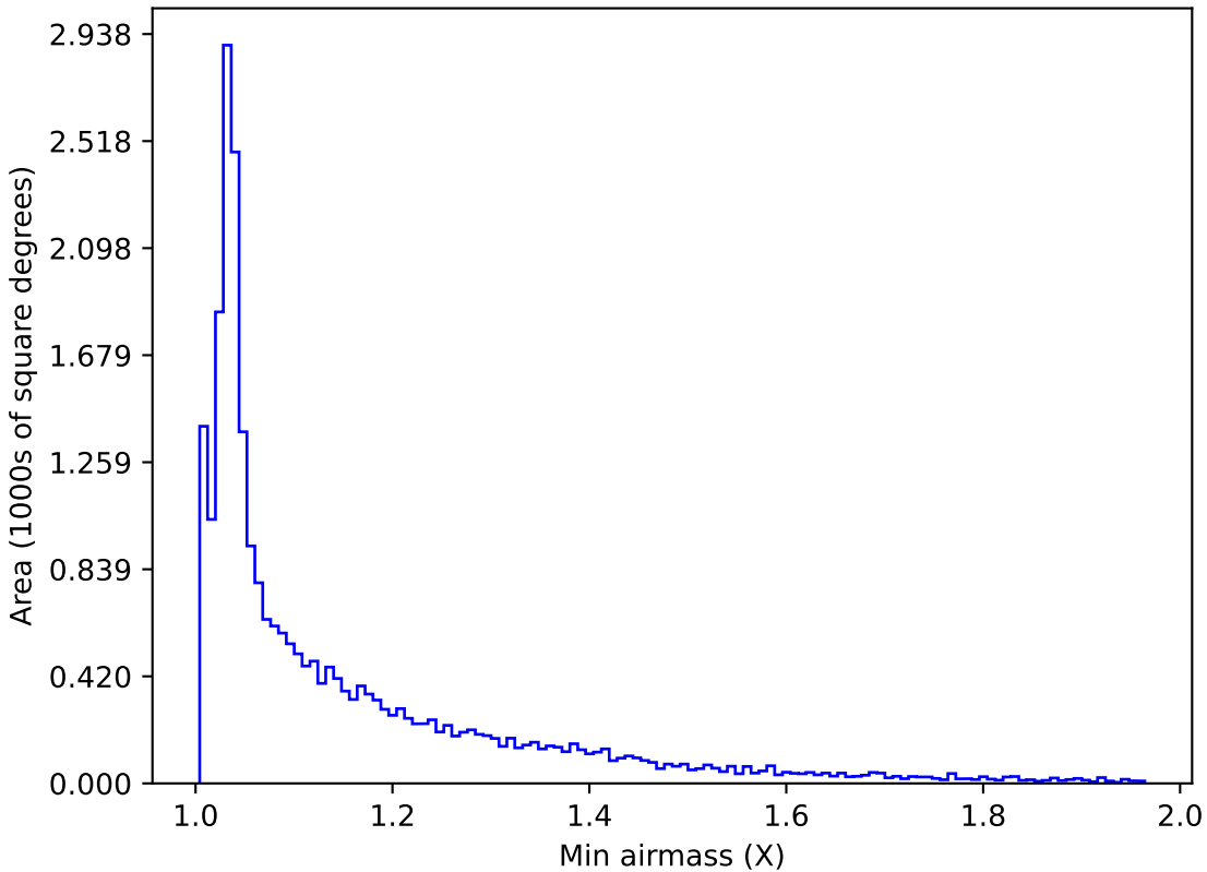
too_elab_r256_d3_griz_v3.4_10yrs All sky g band: Min airmass
