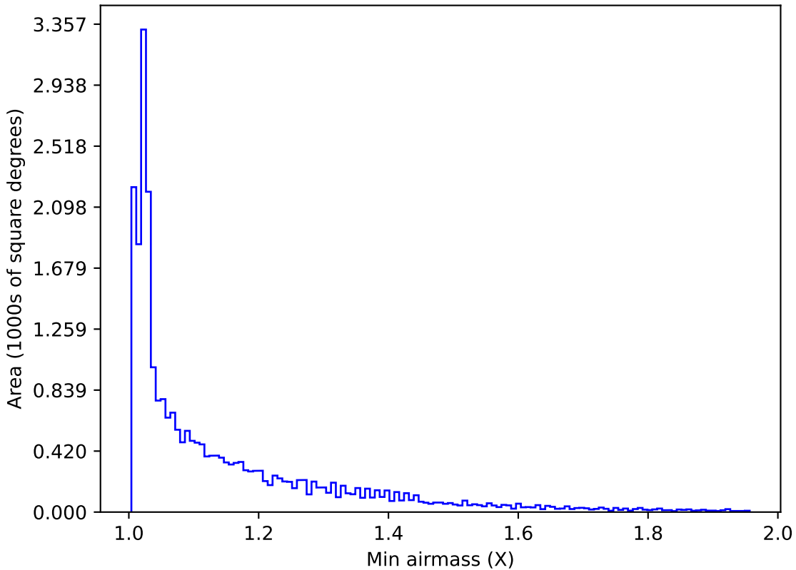
too_elab_r256_d3_griz_v3.4_10yrs All sky all bands: Min airmass
