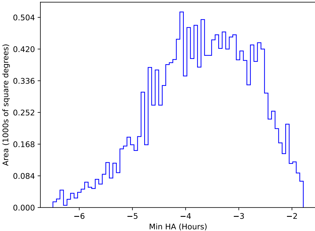
too_elab_r256_d3_griz_v3.4_10yrs WFD y band: Min HA
