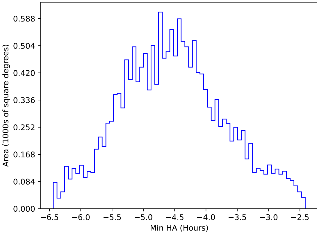
too_elab_r256_d3_griz_v3.4_10yrs WFD r band: Min HA
