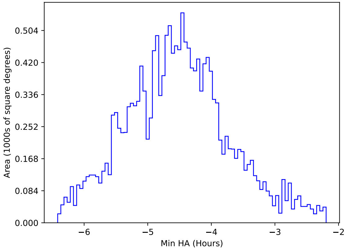
too_elab_r256_d3_griz_v3.4_10yrs WFD i band: Min HA
