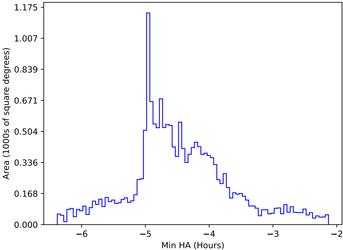
too_elab_r256_d3_griz_v3.4_10yrs WFD g band: Min HA
