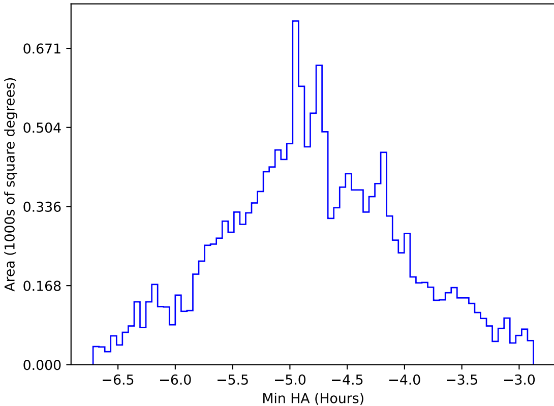
too_elab_r256_d3_griz_v3.4_10yrs WFD all bands: Min HA
