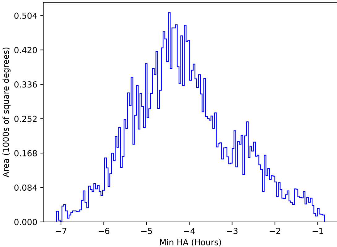
too_elab_r256_d3_griz_v3.4_10yrs All sky z band: Min HA
