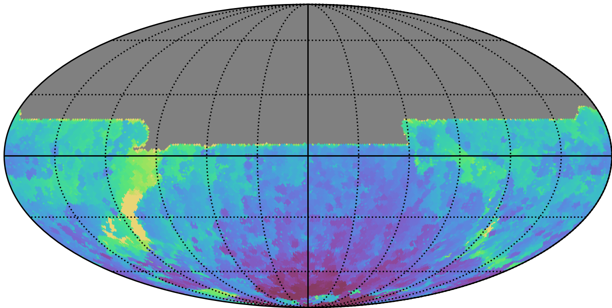
too_elab_r256_d3_griz_v3.4_10yrs All sky y band: Min HA
