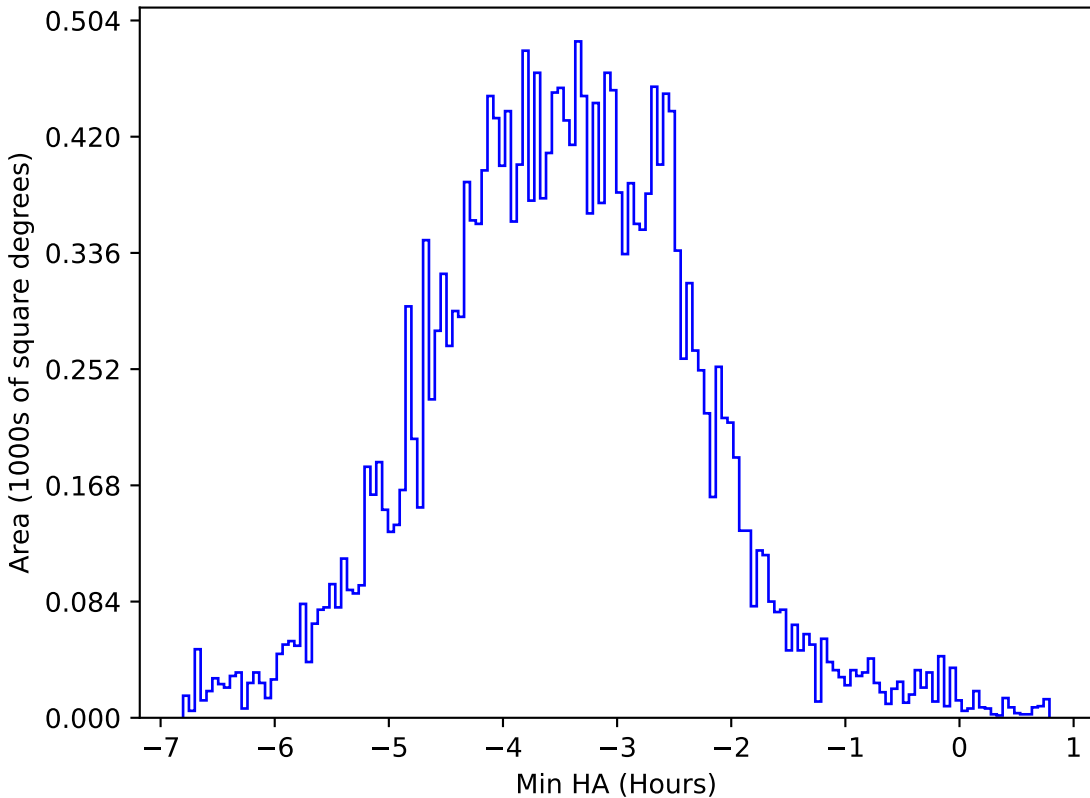
too_elab_r256_d3_griz_v3.4_10yrs All sky y band: Min HA
