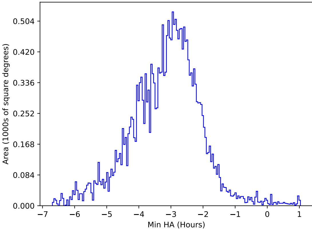
too_elab_r256_d3_griz_v3.4_10yrs All sky u band: Min HA
