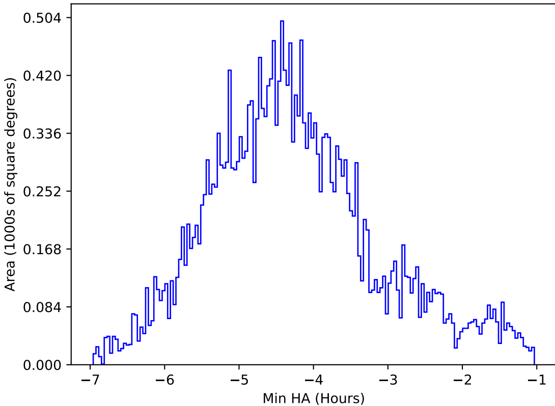
too_elab_r256_d3_griz_v3.4_10yrs All sky r band: Min HA
