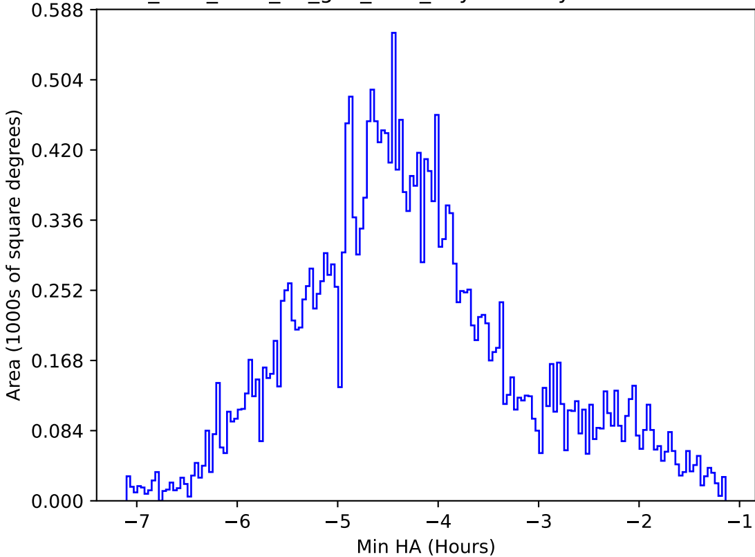
too_elab_r256_d3_griz_v3.4_10yrs All sky i band: Min HA
