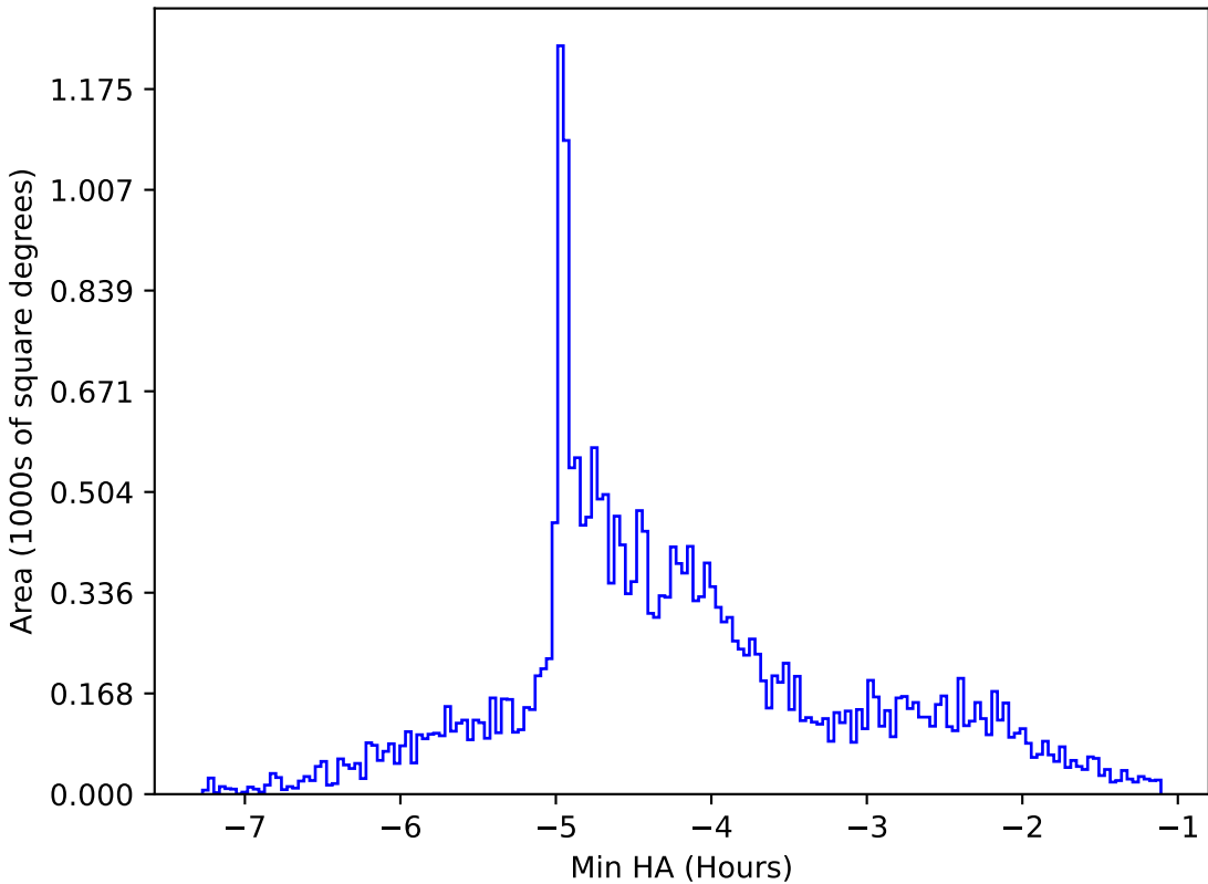
too_elab_r256_d3_griz_v3.4_10yrs All sky g band: Min HA
