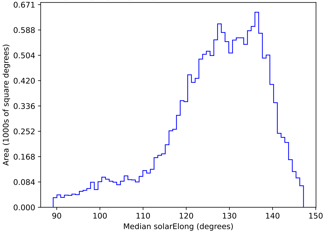
too_elab_r256_d3_griz_v3.4_10yrs WFD z band: Median solarElong
