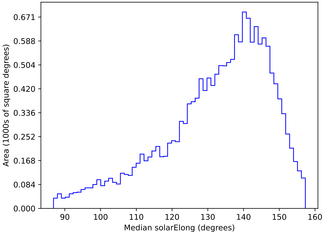
too_elab_r256_d3_griz_v3.4_10yrs WFD u band: Median solarElong
