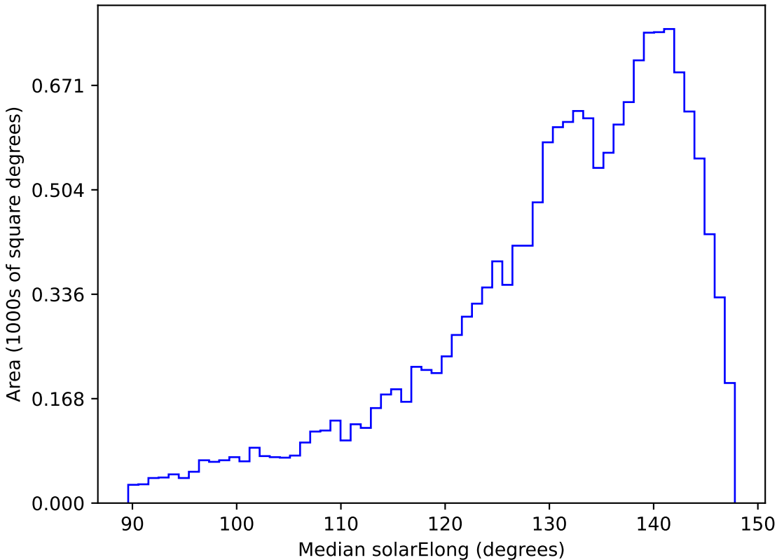
too_elab_r256_d3_griz_v3.4_10yrs WFD r band: Median solarElong
