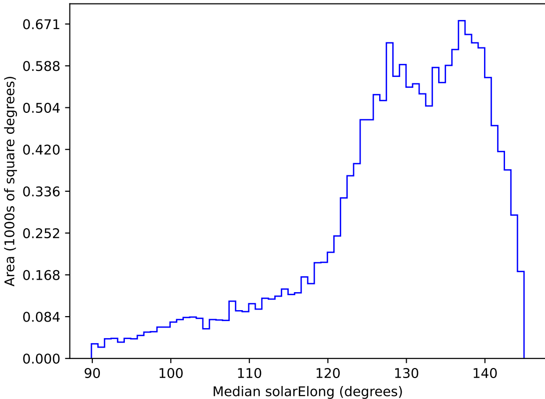
too_elab_r256_d3_griz_v3.4_10yrs WFD i band: Median solarElong
